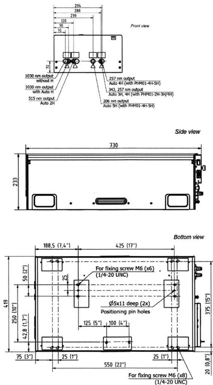
Fig 2. PH2 dimensions.
